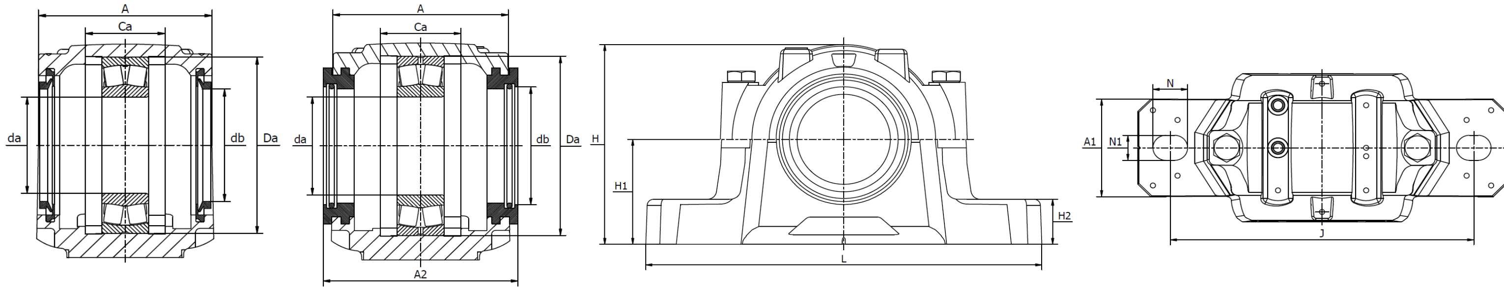
Felt seal, Rubber seal and V-ring seal
