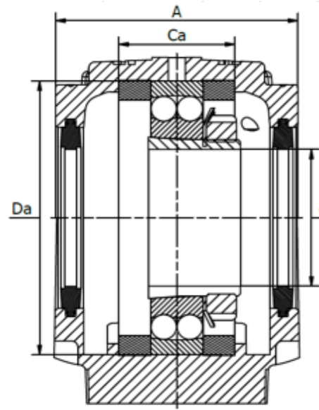
Felt seal, Rubber seal and V-ring seal
