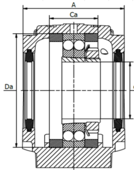
Felt seal, Rubber seal and V-ring seal
