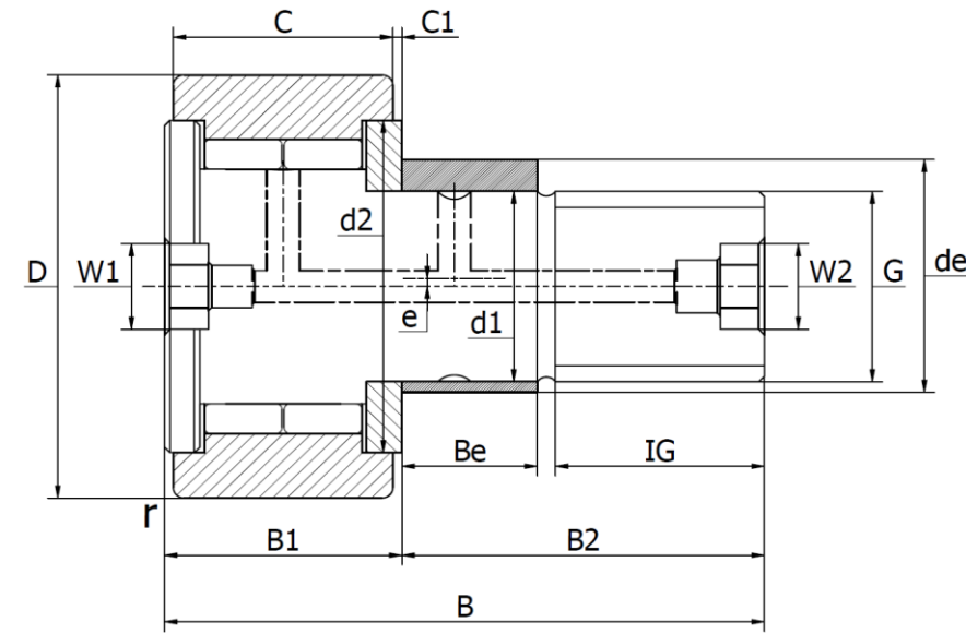
Size 47 to 90
