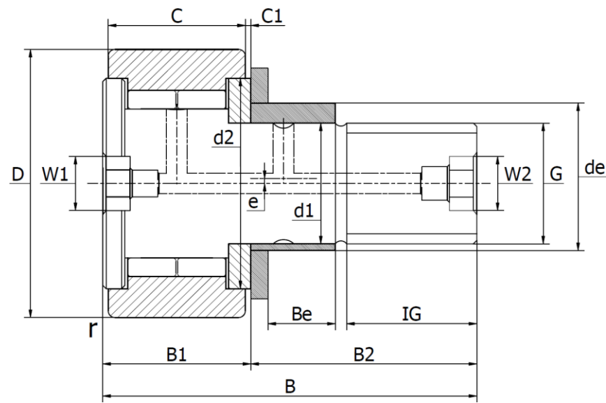
Size 35 & 40
