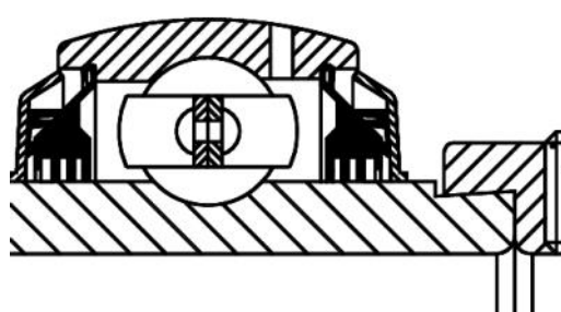
R6 Seal
