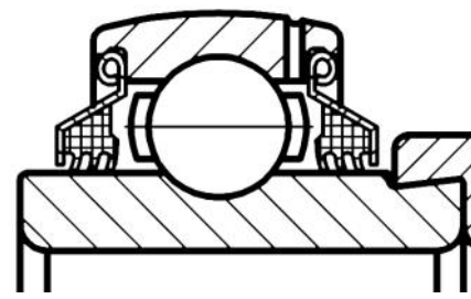
R3 Seal
