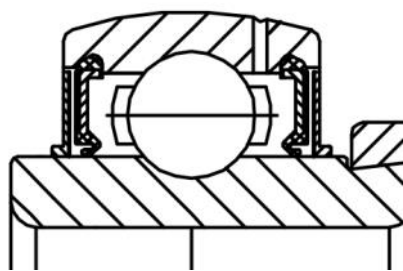
2RS Seal
